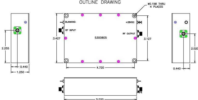
OUTLINE DRAWING
